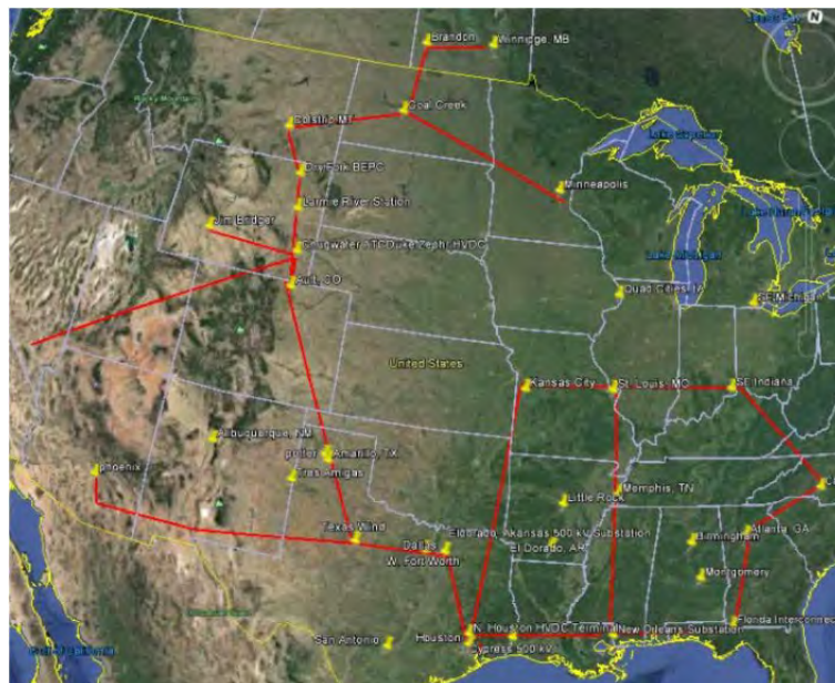
Figure 3 Conceptual National HVDC Network
